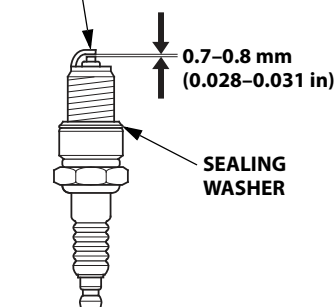
SIDE ELECTRODE
